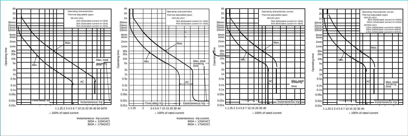
NF250-UGV
