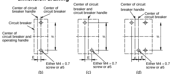
Type names Applicable models Drilling plans Dimensions (mm) Trip button position Mounting screws A Fixed type B Adjustable type(*1) D E F Number of poles Number of poles C (min.) C (max.) V-05SV2 NF32-SV 2 — — (b) (a) 39 125 — — 12.5 111 H (a): Breaker mounting screws (2 pcs) (4 pcs for 4P) V-05SVE2 NF63-CV, NF63-SV, NF63-HV V-05SV NF125-SVF 2/3 NV32-SV 2/3 (c) (a) V-05SVE NF32-SV 3 NV63-CV, NV63-SV, NV63-HV 162 300 25 J NF63-CV, NF63-SV, NF63-HV 4 — — (d) (a) V-1SV2 NF125-CV, NF125-SV 2 — — (b) (a) — — 15 H (b): Breaker - operating handle mounting screws and nuts (2 pcs each) V-1SVE2 V-1SV NF125-CV, NF125-SV 3 NV125-CV, NV125-SV, NV125-HV 3 (c) (a) V-1SVE NF63-HRV, NF125-HV 4 4 (d) (a) 30 J 2/3 — — (c) (a) 4 (d) (a) V-2SV NF125-SEV, NF125-HEV, NF125-SGV 2/3 NV125-SEV, NV125-HEV 3 (c) (a) 41 162 300 90 35 126 K V-05SV2, V-05SVE2, V-1SV2 and V-1SVE2 use (b) only with no nuts attached. V-2SVE NF125-LGV, NF125-HGV, NF125-RGV NF160-SGV, NF160-LGV, NF160-HGV NF250-CV, NF250-SV, NF250-HV NV250-CV, NV250-SV, NV250-HV NF250-SGV, NF250-LGV, NF250-HGV NF250-SEV, NF250-HEV, NF250-RGV 4 NV250-SEV (*2), NV250-HEV (*2) 4 (d) (a)
